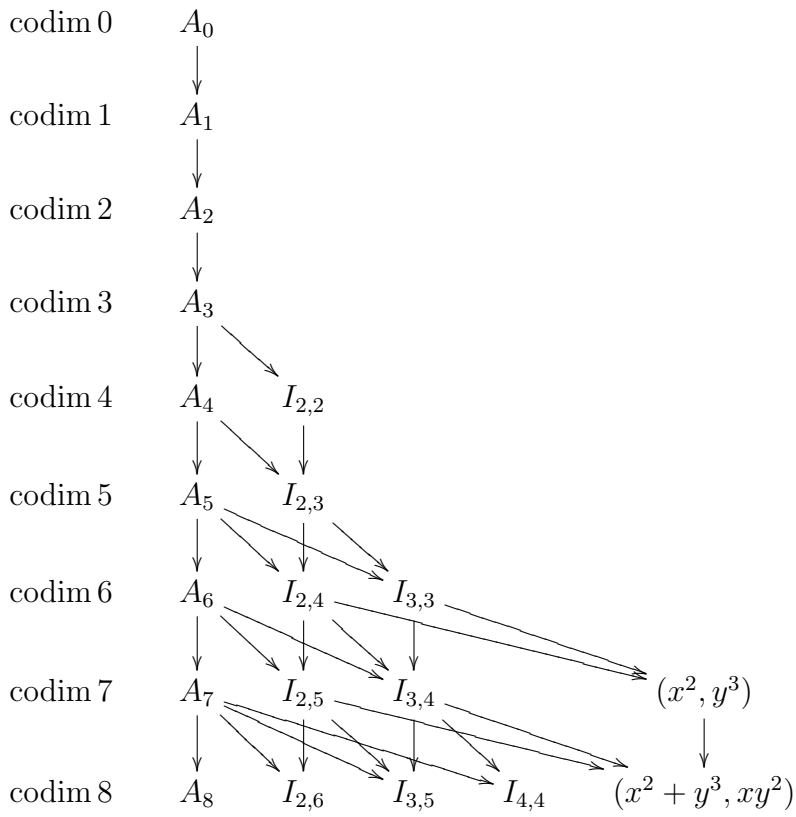
FIGURE 1. The hierarchy of l = 0 contact singularities, upto codimension 8
