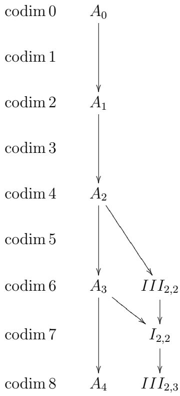
FIGURE 1. The hierarchy of l = 1 contact singularities, upto codimension 8
